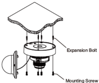
Figure 2-2 fix the camera onto wall/ceiling
