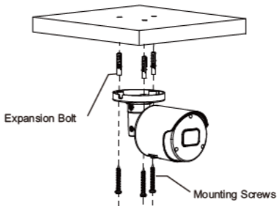
Figure 2-1 Fix the camera on wall/ceiling
