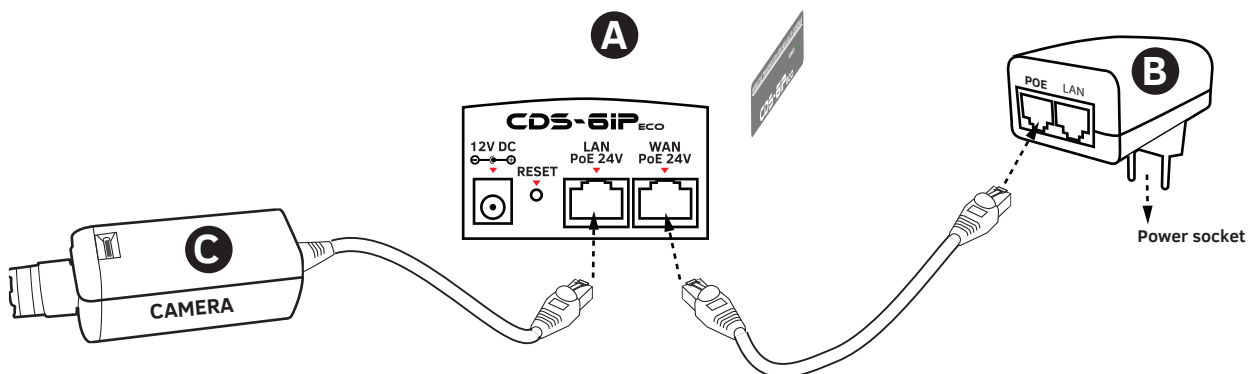
Scheme 2. Option 1 devices connection
