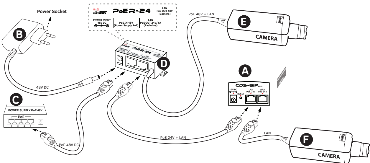
Scheme 5. Option 4 devices connection
