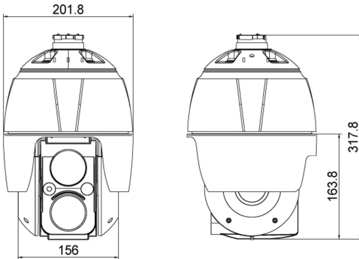
Dimensions: mm
