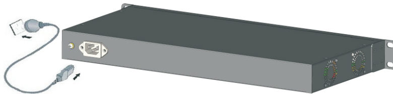
Figure 2-6 Connect power cable
